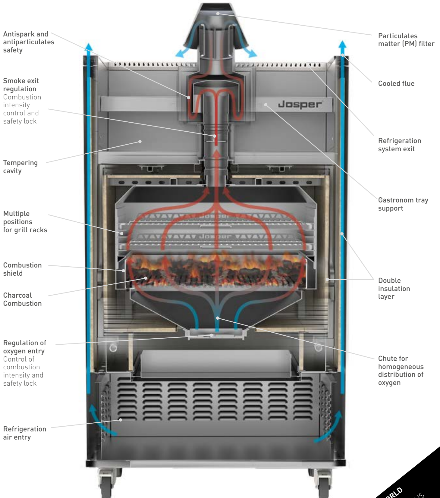
Josper Charcoal Broiler Oven A Class - Model HJA-50
