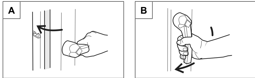
Image: Closing the two-stage door latch
